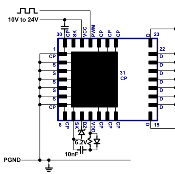
Fig. 18. Start-up circuit
