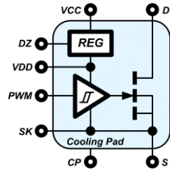
Simplified schematic
